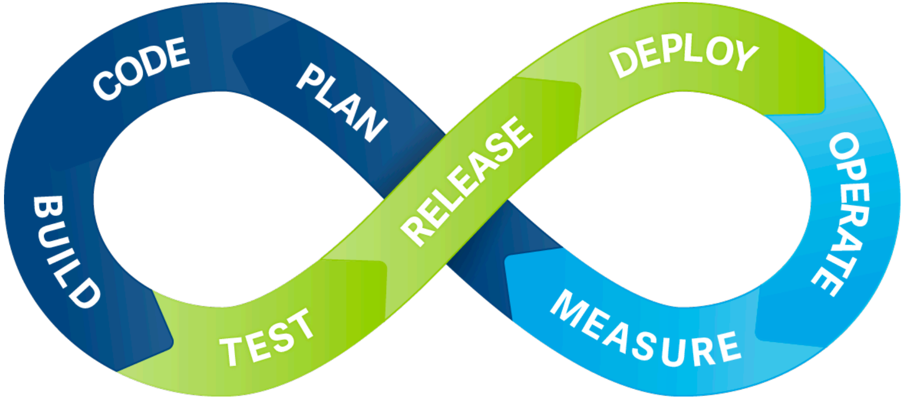
Continuous Deployment?
